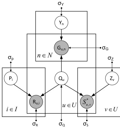
Fig. 4. Graphic model of Weibo-MF.
